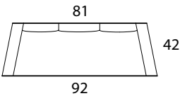
Sofa / 2A 2-Arm Sofa
